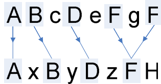
Figure 1: The Pinheiro and Sun similarity metric alignment for the strings \sigma_1 = ABcDeFgH \sigma_2 = AxByDzF .
