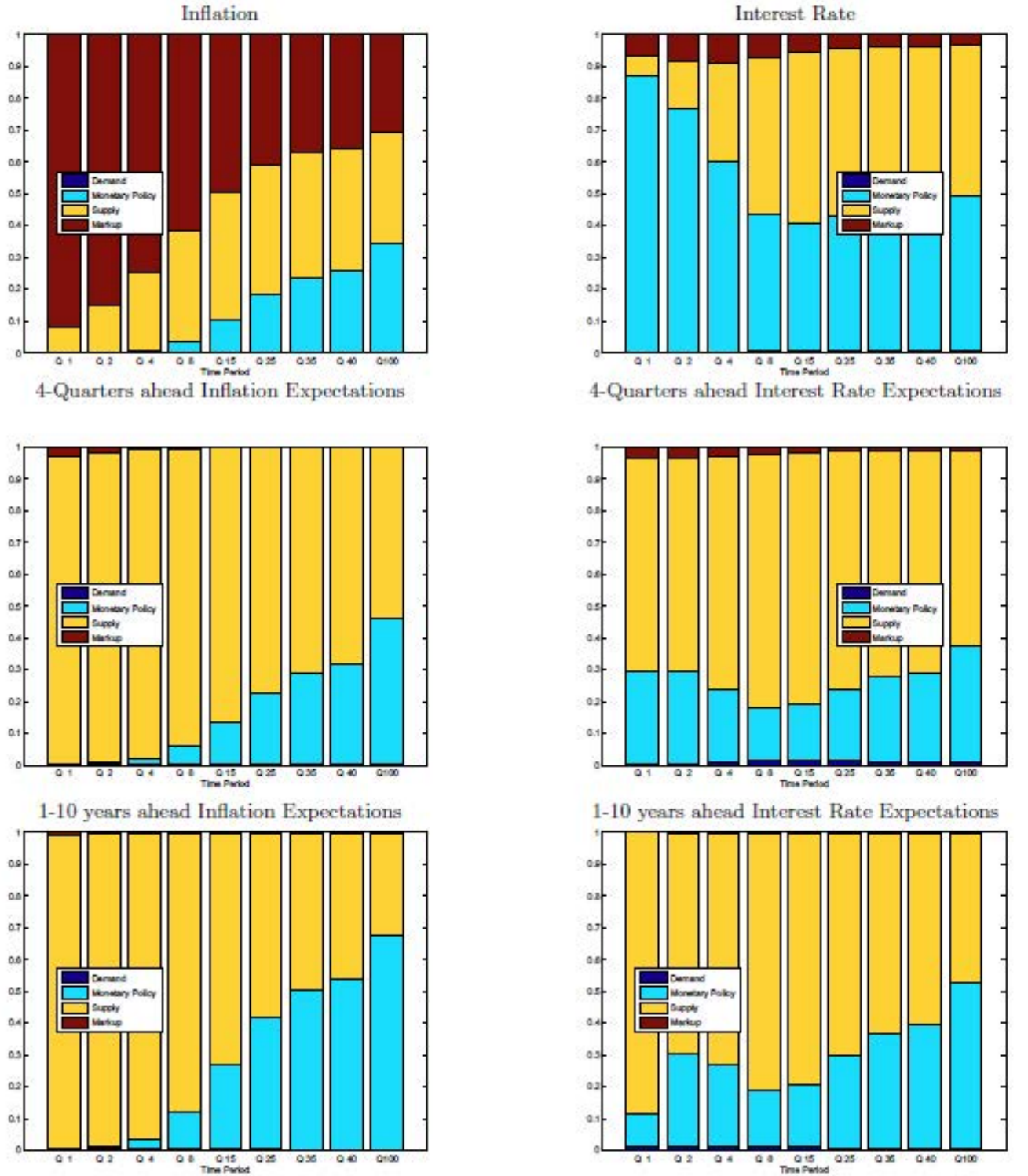
Figure 6: Variance Decomposition
